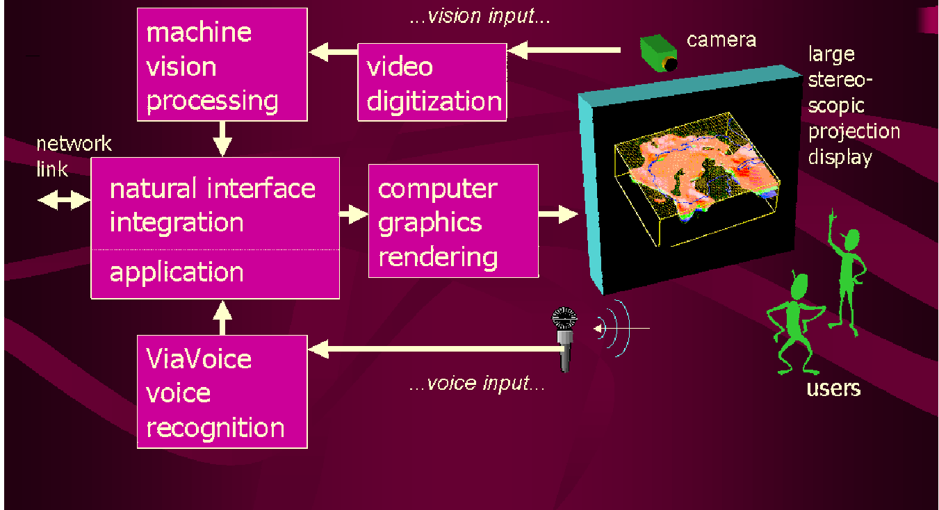
Figure 1: A schematic of the Visualization Space. The two input channels – voice and vision – are combined to control applications running on a single IBM PC. Visual output is displayed on a large projection display.
